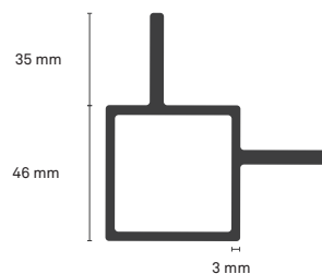
Corner connector
