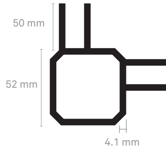
Corner connection
