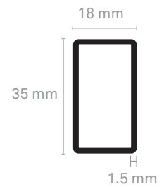
Truss part
